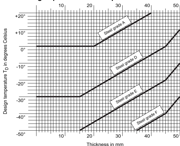
Figure 5 : Steel selection for first category high strength quenched and tempered elements
