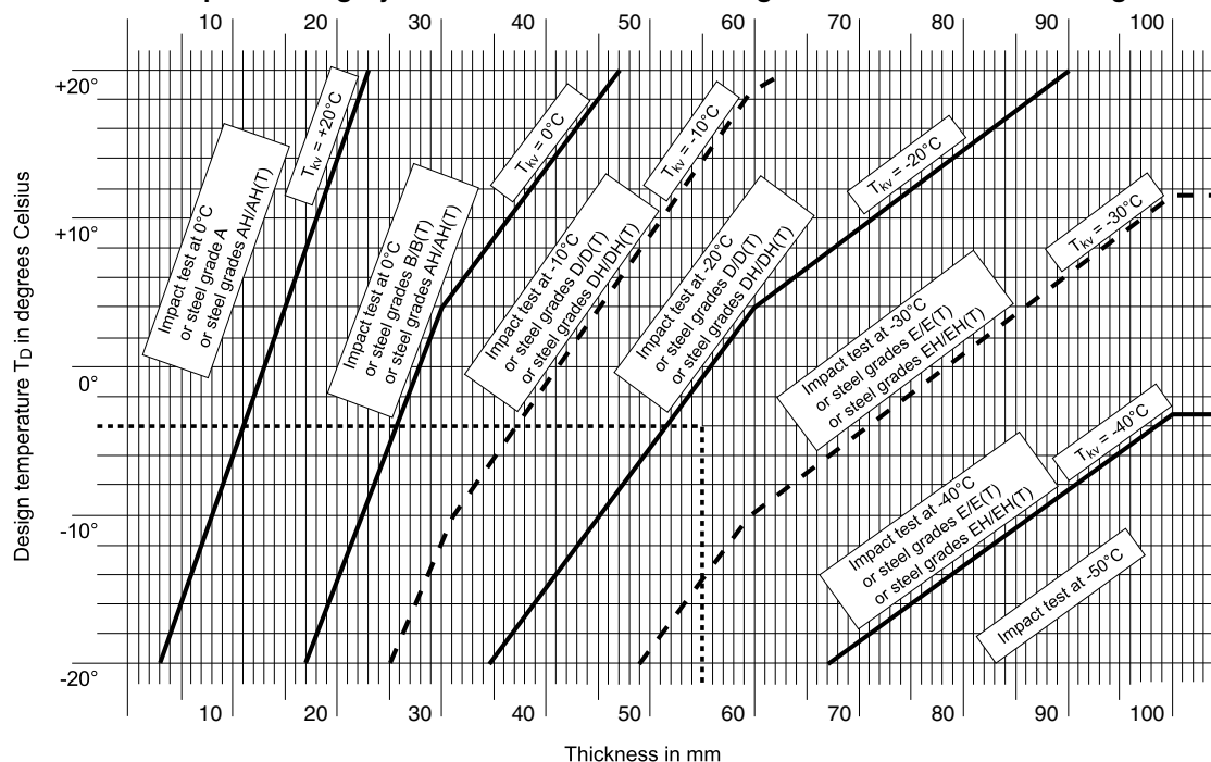
Figure 2 : Steel selection for first category elements as welded without stress-relieving heat treatment after welding or for special category elements with stress-relieving heat treatment after welding
