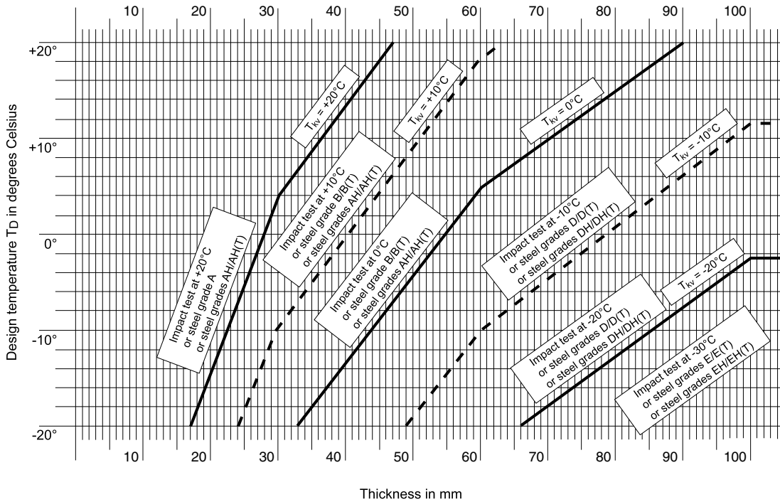
Figure 3 : Steel selection for second category elements with or without stress-relieving treatment after welding or first category elements with stress-relieving heat treatment after welding
