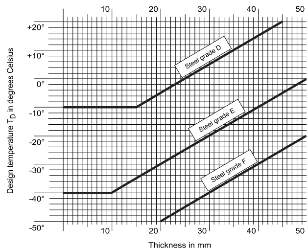
Figure 4 : Steel selection for special category high strength quenched and tempered elements
