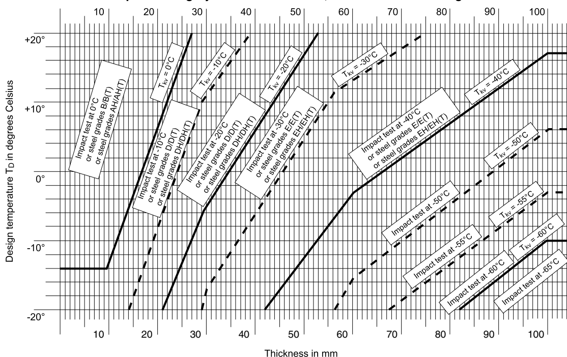
Figure 1 : Steel selection for special category elements as welded, without stress-relieving heat treatment after welding
