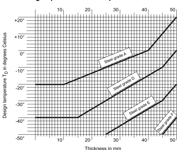
Figure 6 : Steel selection for second category high strength quenched and tempered elements
